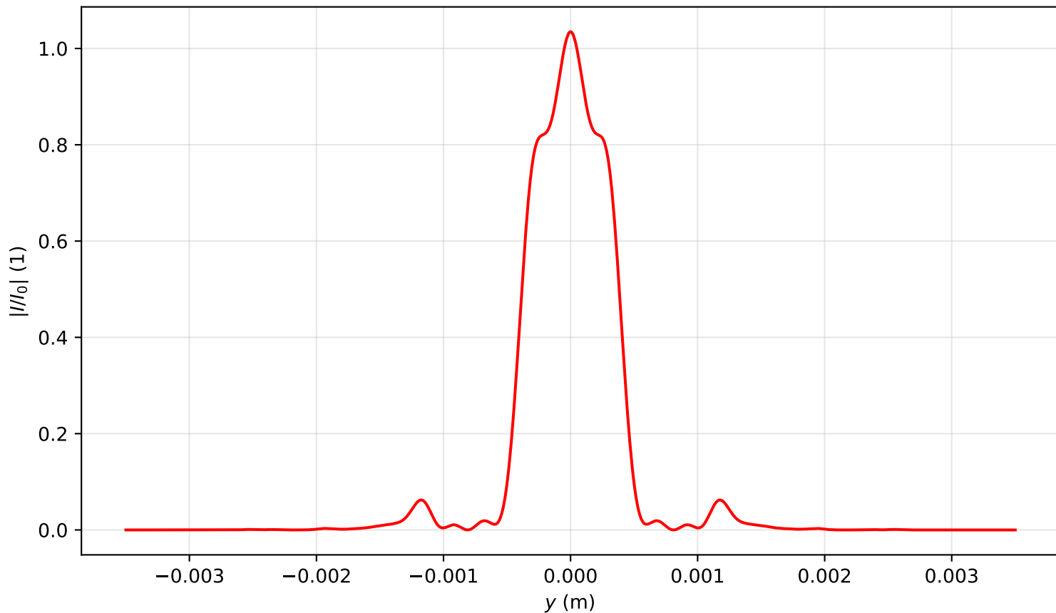
Intensity profile I(x=0, y, z=1.672)/I_0 , P_{in}=4.0P_{cr} , artificial time
